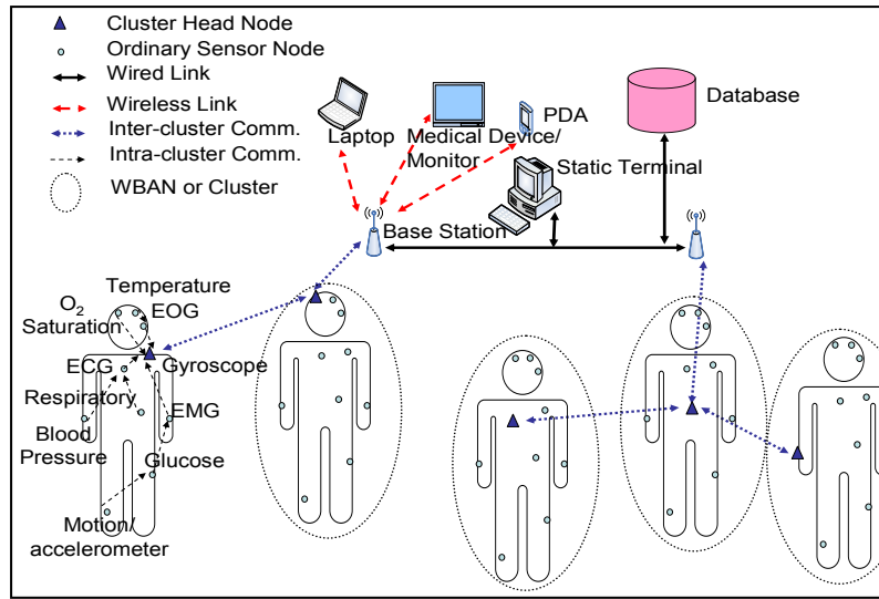
Wireless Information Patient System (WIPS)
