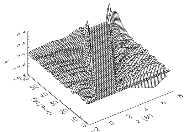
FIG. 2. Normalized Hamiltonian constraint, N = (R + K^2 - K^{ij}K_{ij})/(|R| + |K^2| + |K^{ij}K_{ij}|) , along the z axis as a function of time. The flat region shows the location of the excised part of the domain within the hole.
